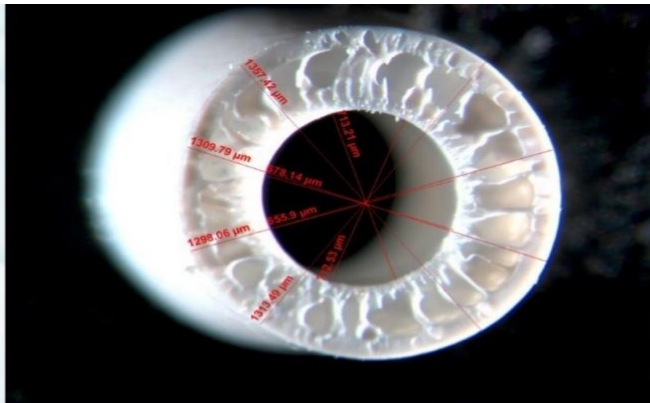
Hollow Fiber
